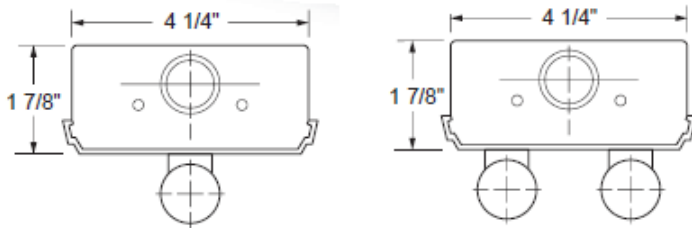
End View 1 and 2 Lamp
