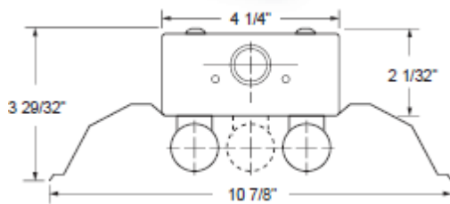
End View – 1 or 2 Lamp
